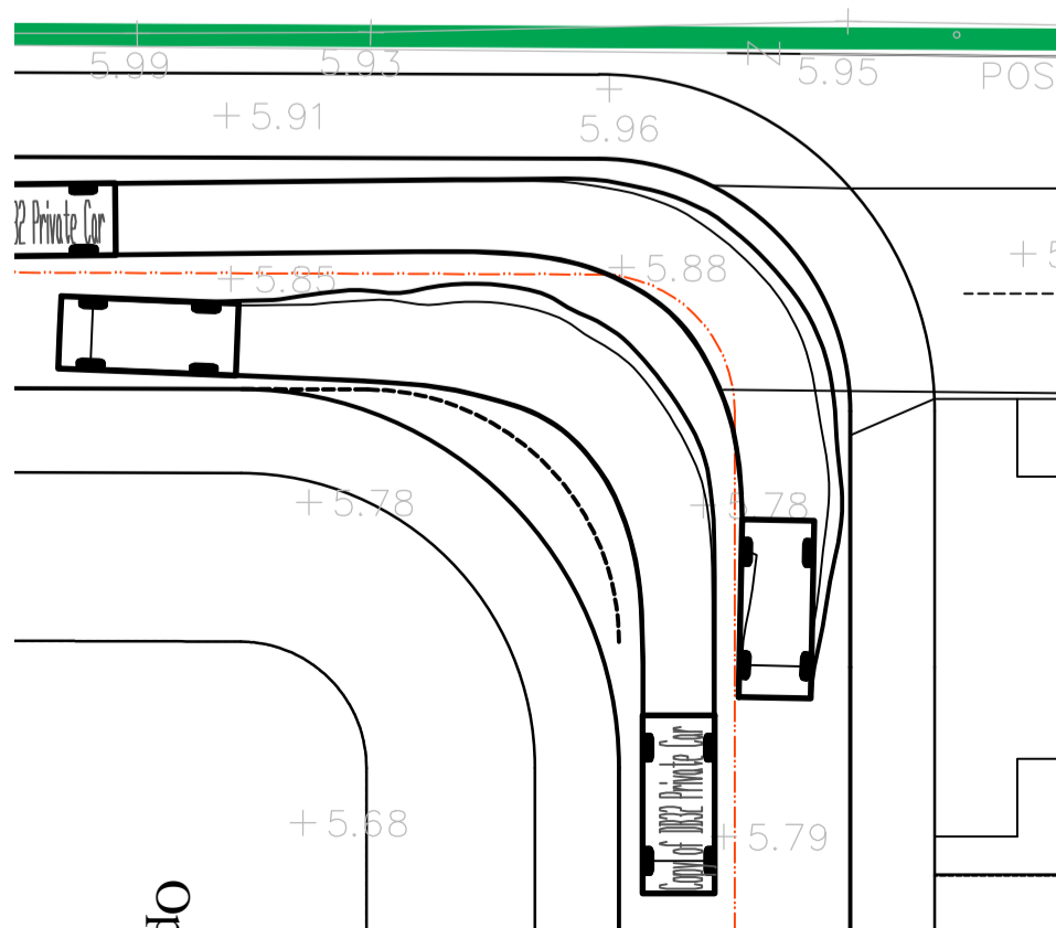
Light Vehicle Swept Path at 90 Degree Bend (1:200)
