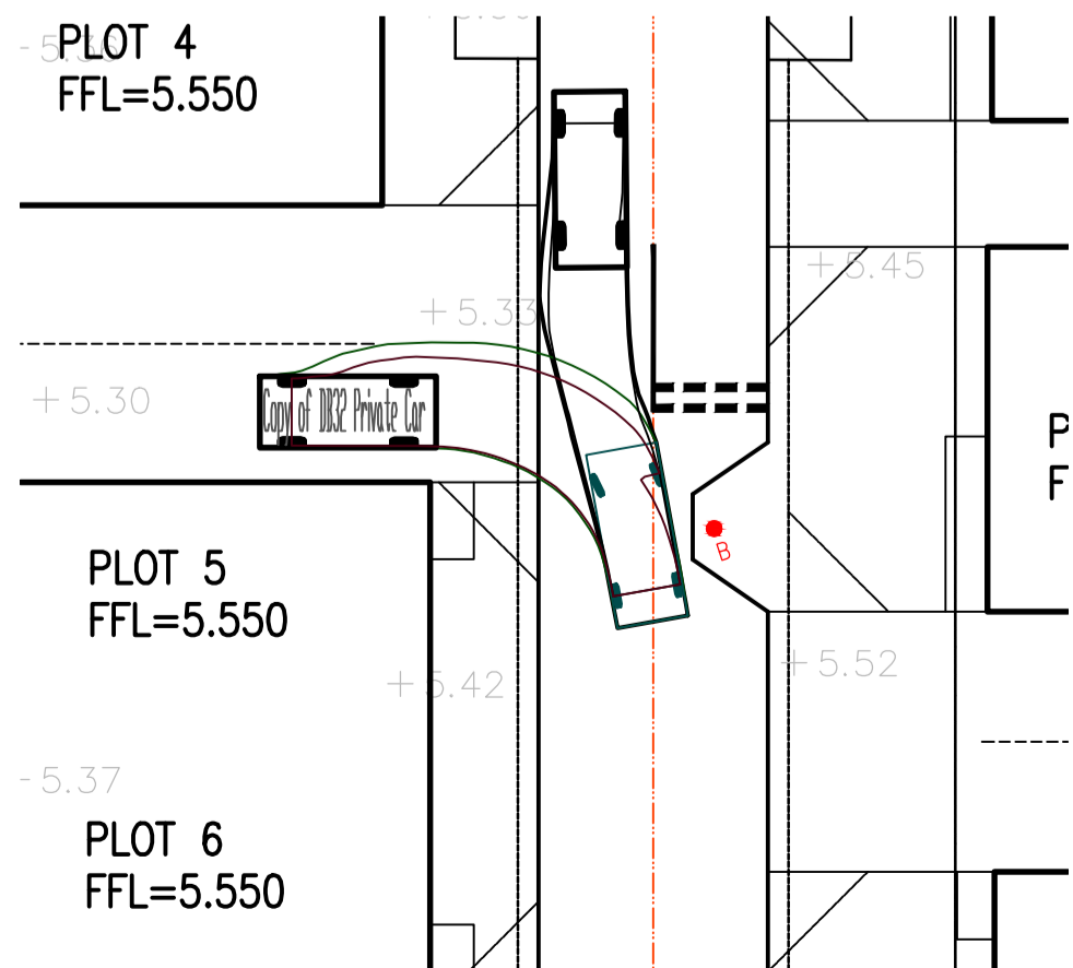
Light Vehicle Swept Path Adjacent to Build Out (1:200)
