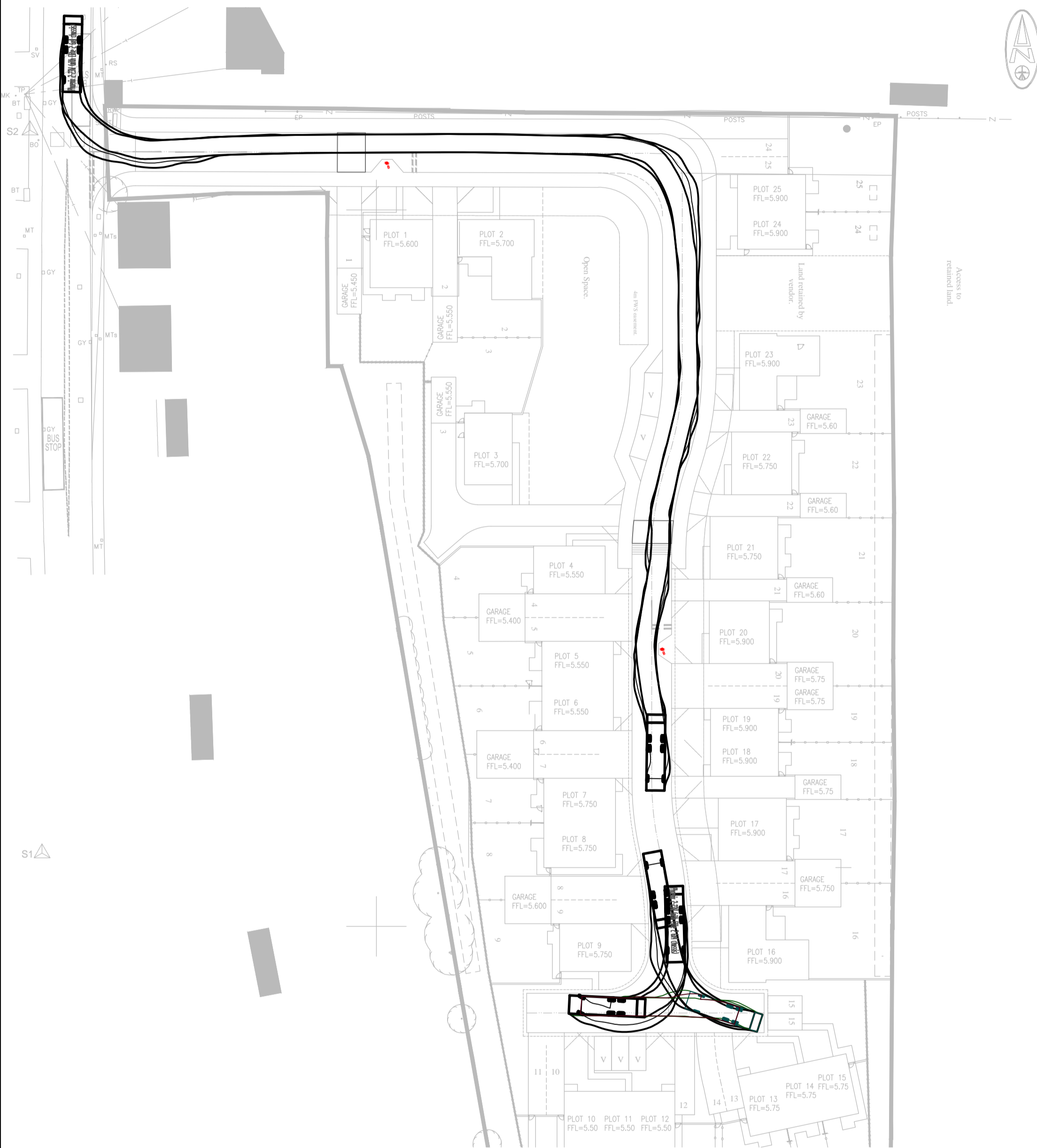
Plan On Refuse Freighter Swept Path (1:500)
